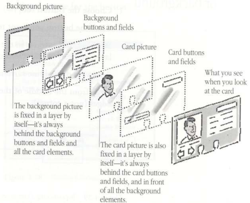
Figure 4-40 HyperCard's layers
