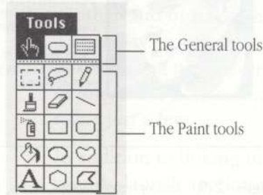
Figure 2-10 HyperCard's tools
