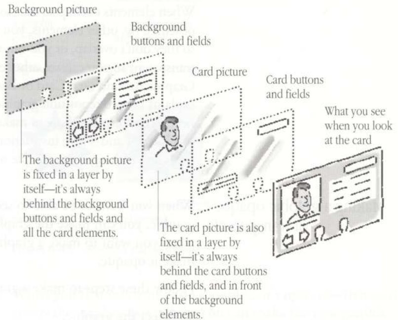
Figure 6-41 HyperCard's layers
