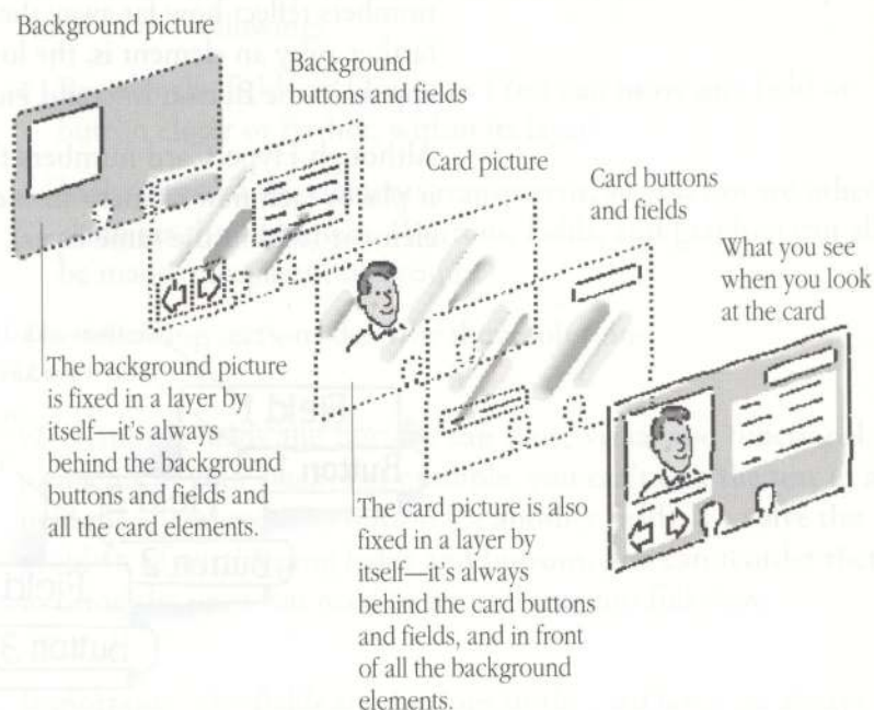
Figure 5-25 HyperCard's layers
