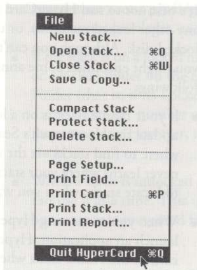
Figure 1-52 Quitting HyperCard
